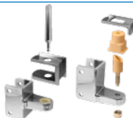
TOP PART ASSEMBLY Part No. 9A3720 Chrome Part No. 9A3043 Cast SS BOTTOM PART ASSEMBLY Part No. 9A3710 Chrome Part No. 9A3033 Cast SS
